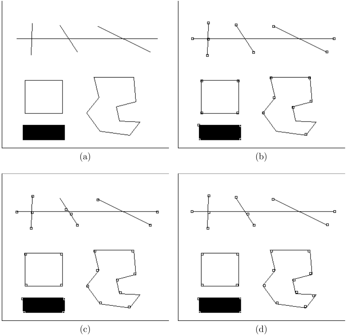
Fig. 7.1 (a) A synthetic image. (b)–(d) Corners detected by Algorithm 3.1 when standard deviation of the Gaussian smoother was 1, 2, and 3 pixels, respectively.
